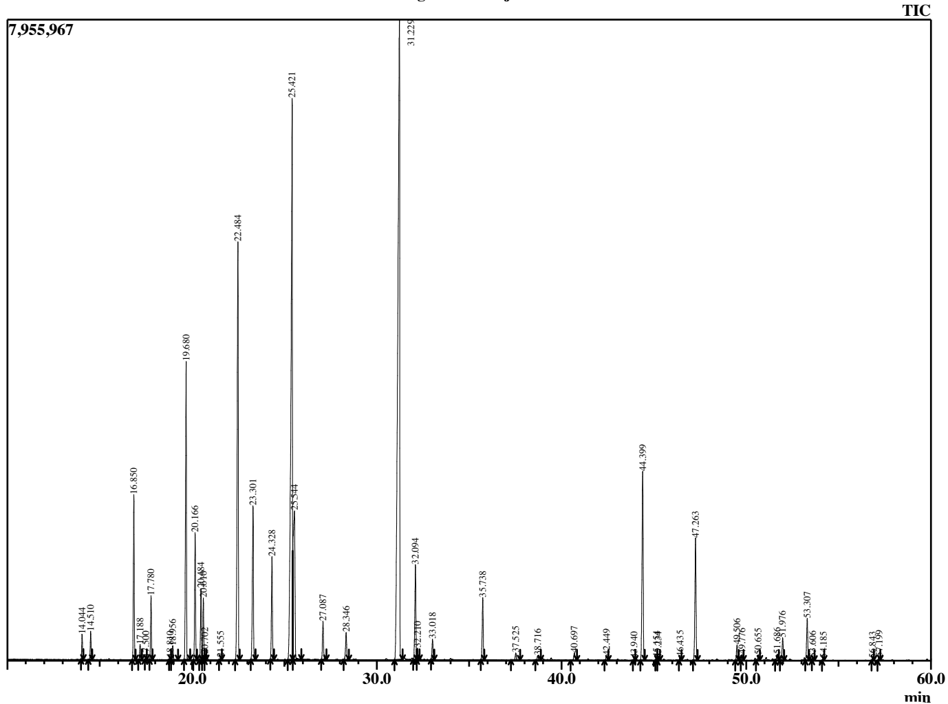
Chromatogram OriMaj2 Lot 23127
